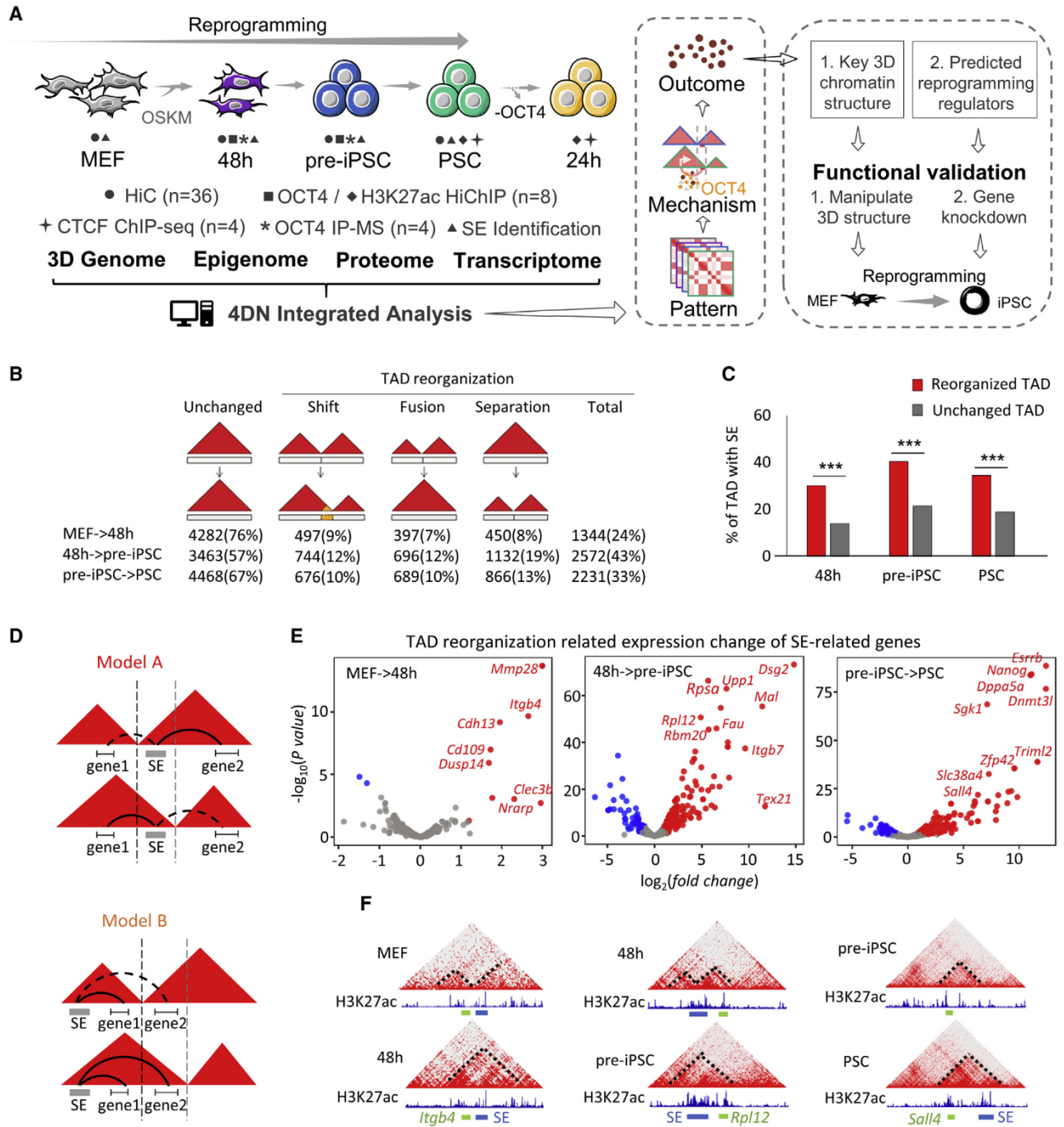
Figure 1. TADs are reorganized during somatic cell reprogramming
